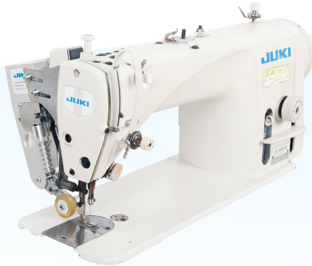
GPB-2 Puller Attachment (for lockstitch) JUKI DDL-8700 /DDL-9000
